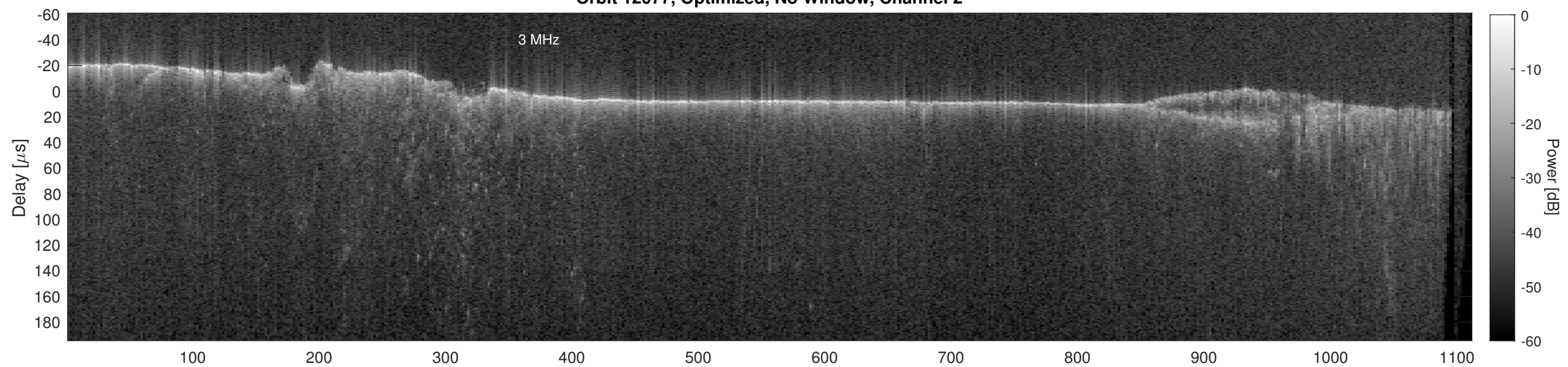
Orbit 12077, Cluttergram
