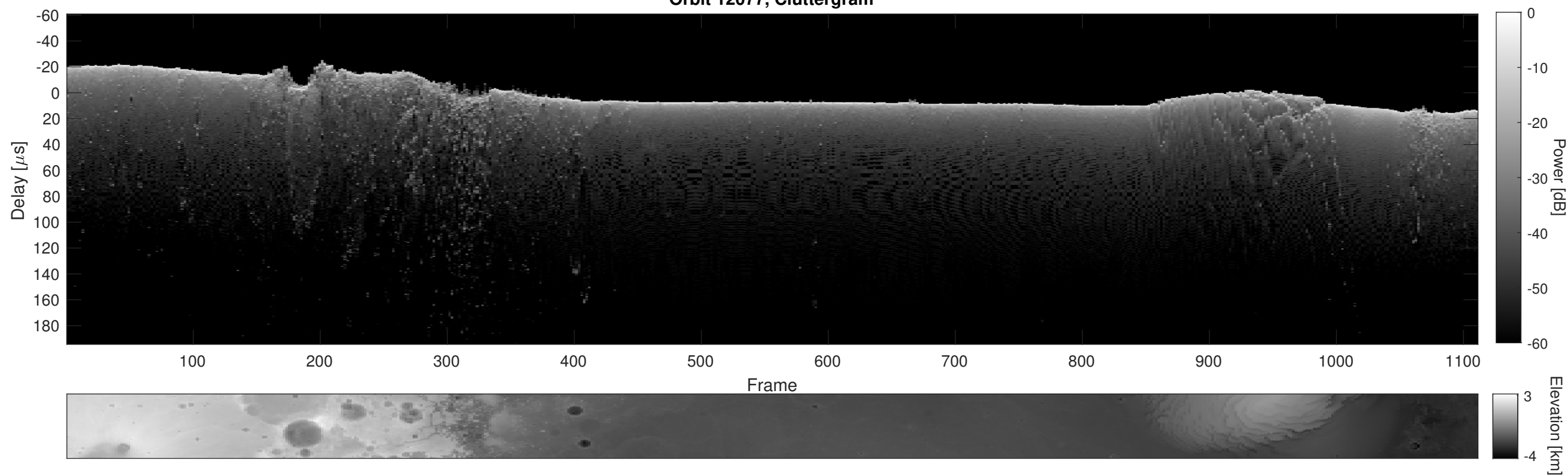
Orbit 12077, Cluttergram
