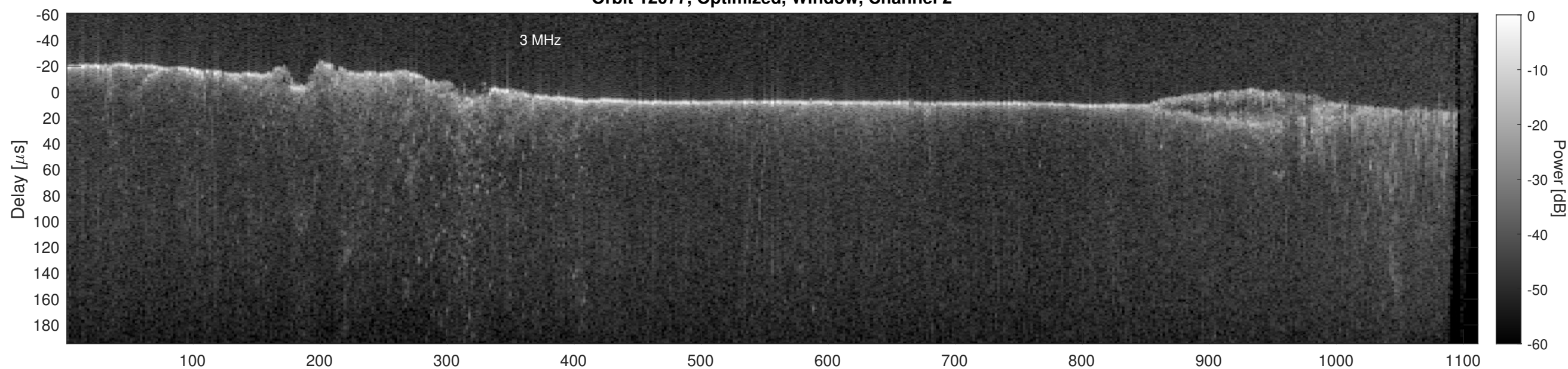
Orbit 12077, Cluttergram
