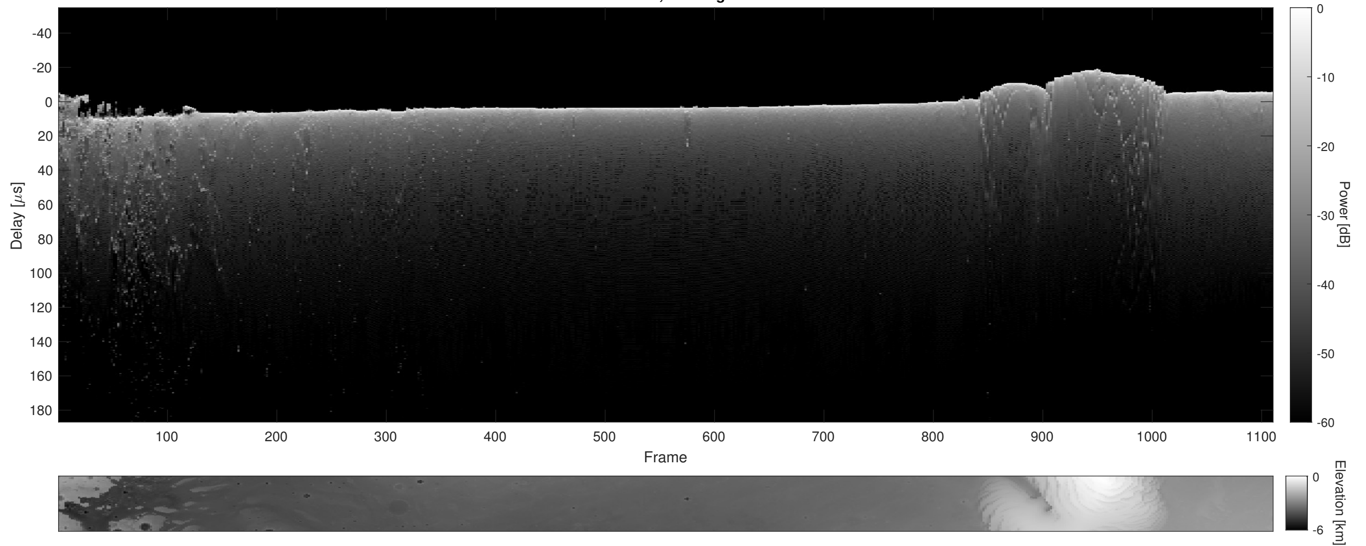
Orbit 12078, Cluttergram
