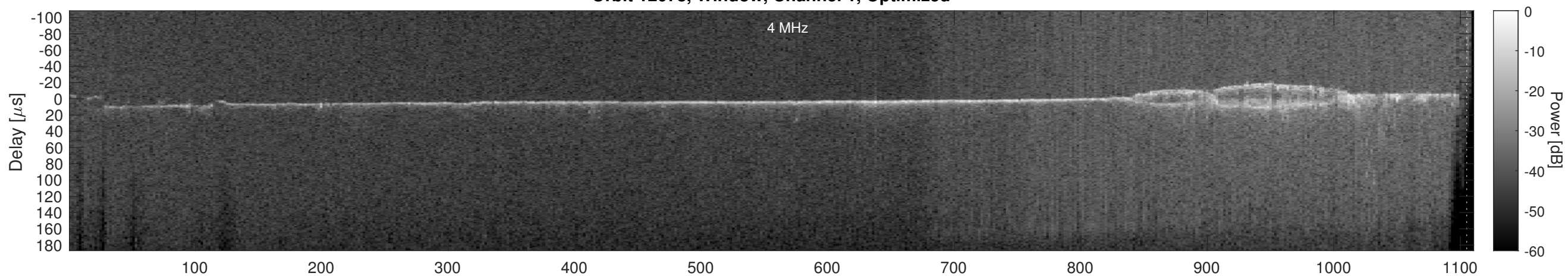
Orbit 12078, Cluttergram
