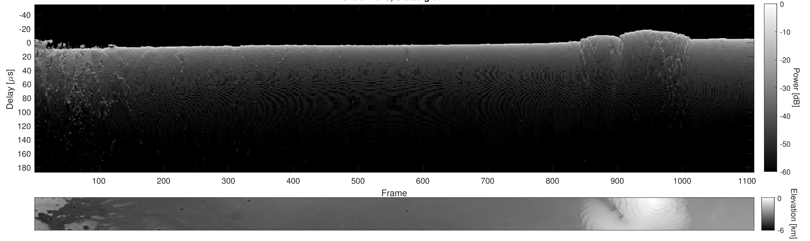
Orbit 12078, Cluttergram
