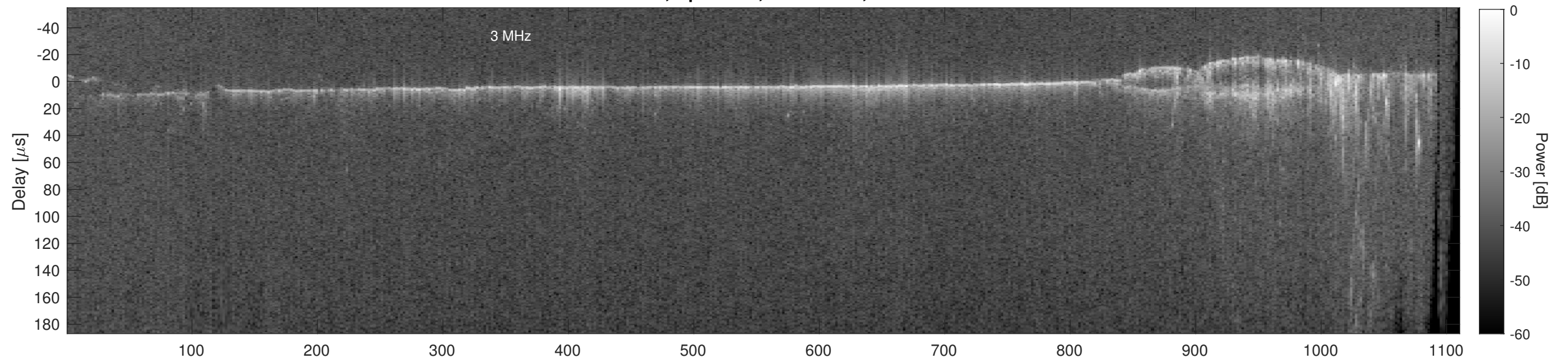
Orbit 12078, Cluttergram
