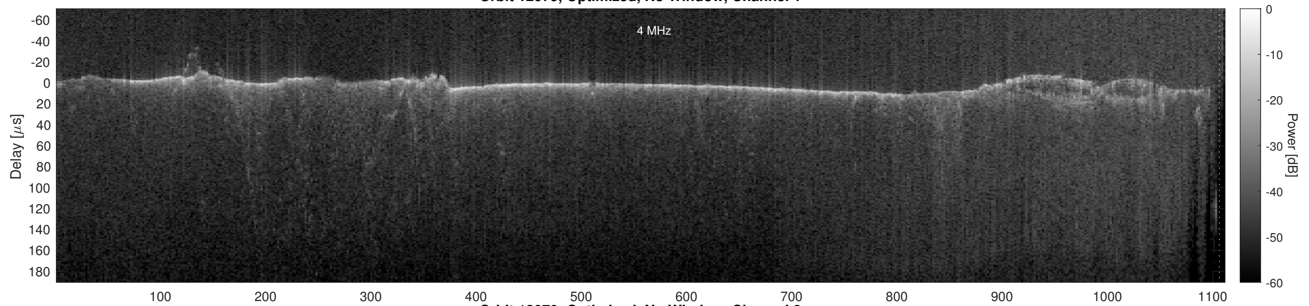
Orbit 12079, Optimized, No Window, Channel 2
