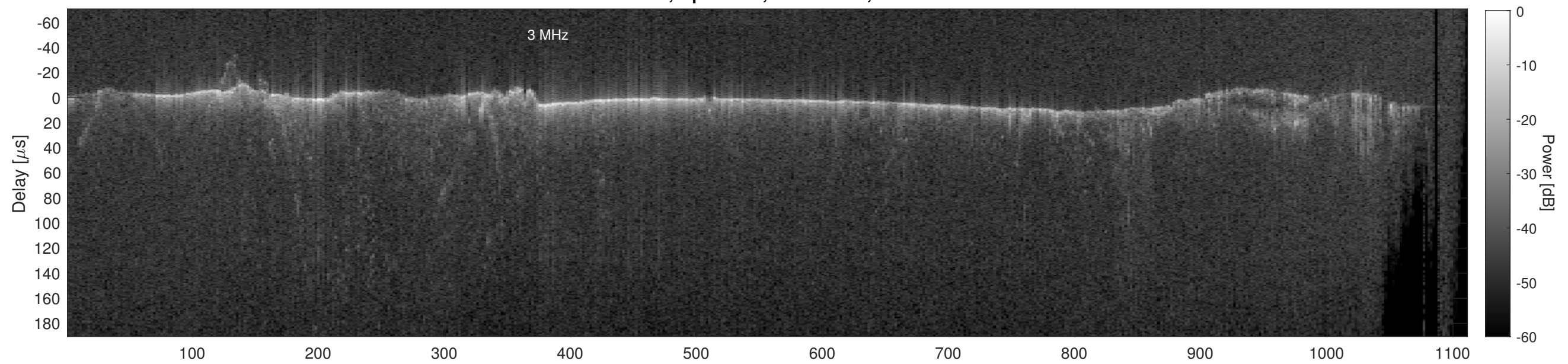
Orbit 12079, Cluttergram
