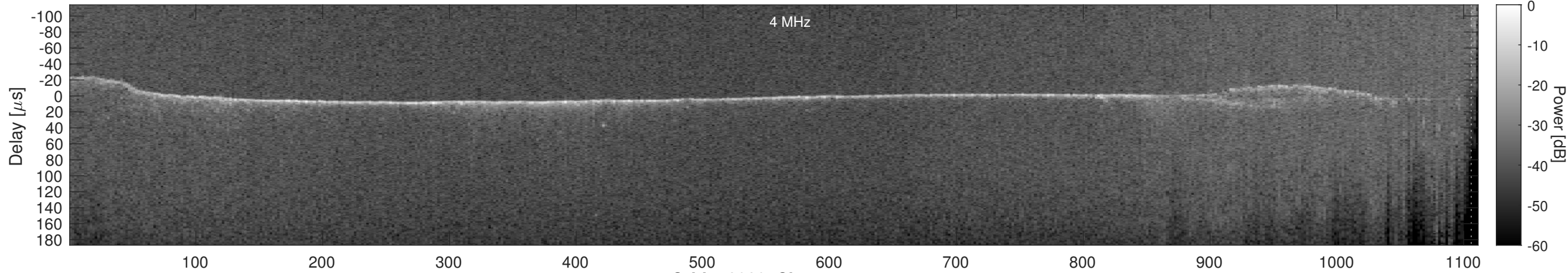
Orbit 12080, Cluttergram
