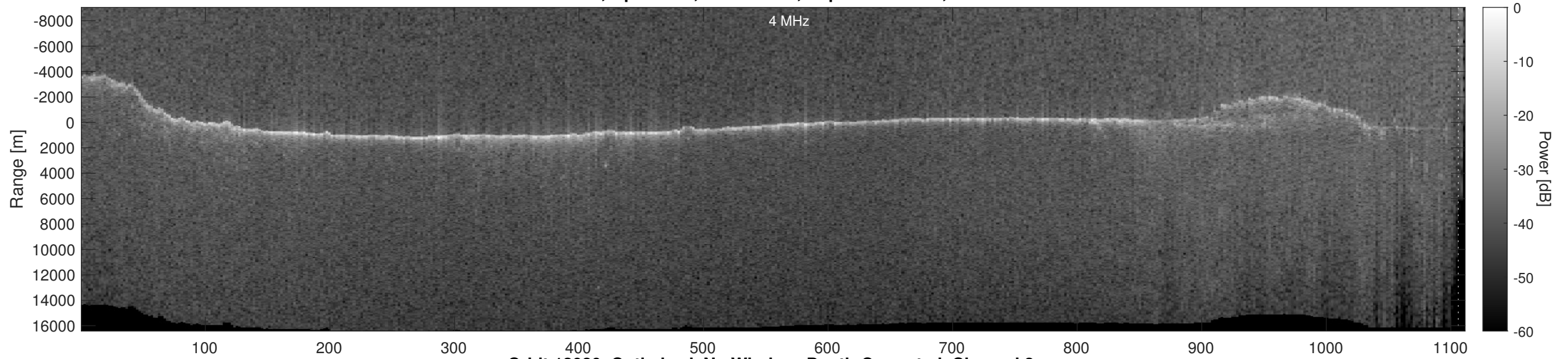
Orbit 12080, Optimized, No Window, Depth-Corrected, Channel 2
