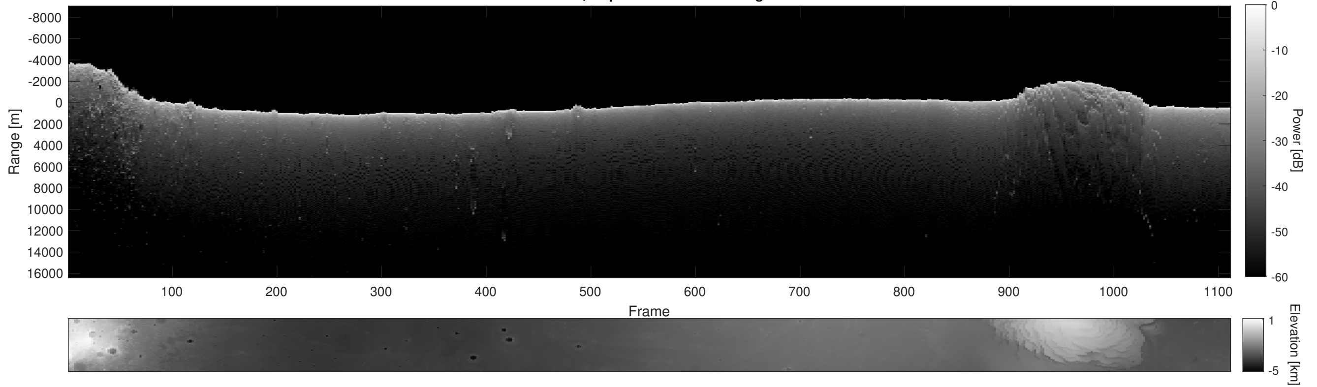
Orbit 12080, Depth-Corrected Cluttergram
