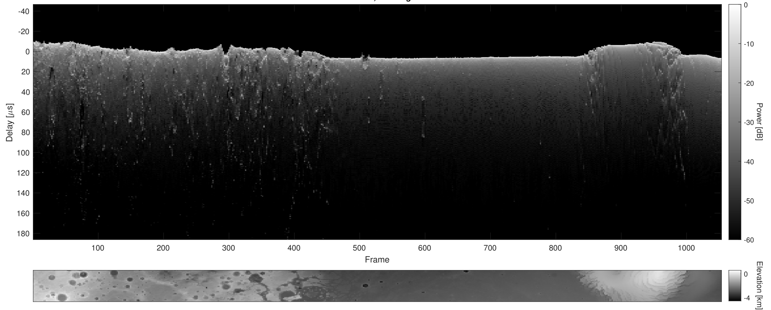
Orbit 12081, Cluttergram
