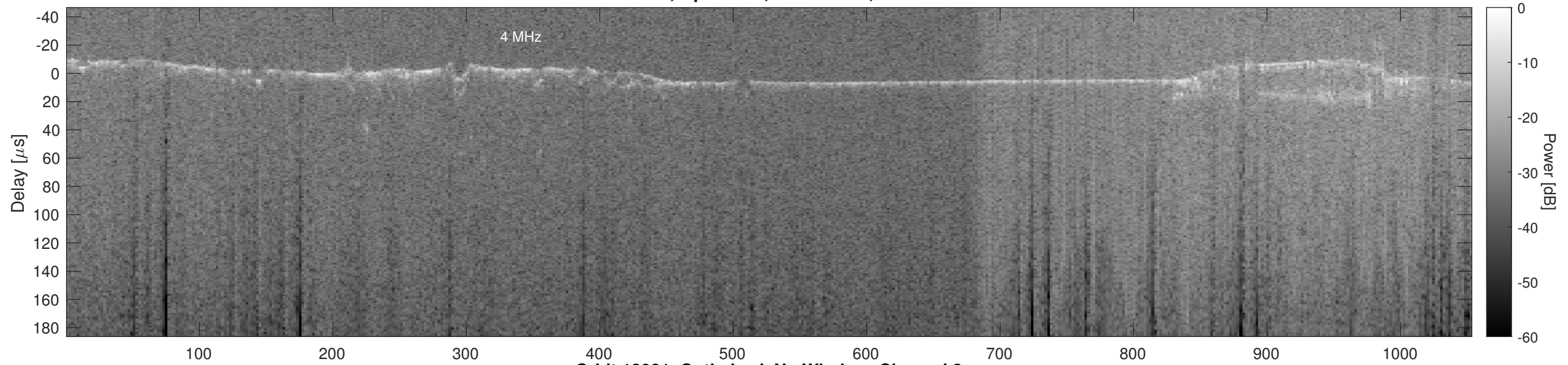
Orbit 12081, Optimized, No Window, Channel 2
