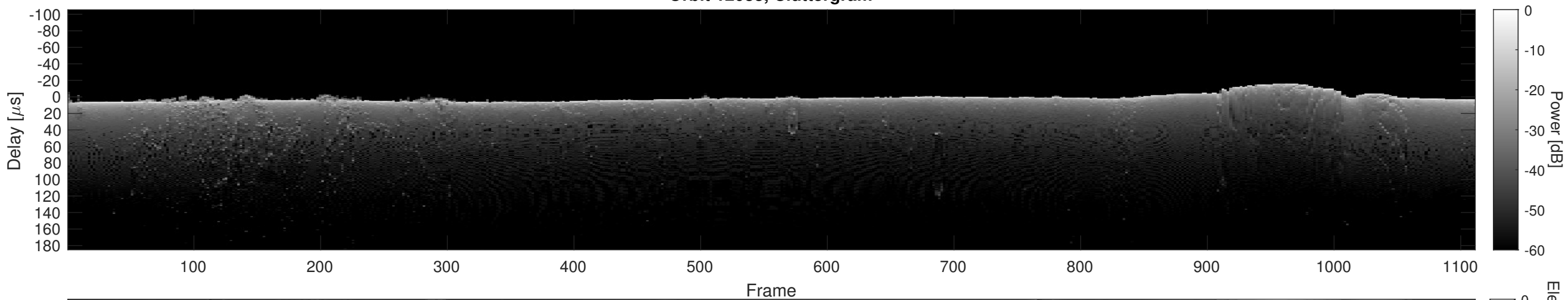
Orbit 12083, Cluttergram
