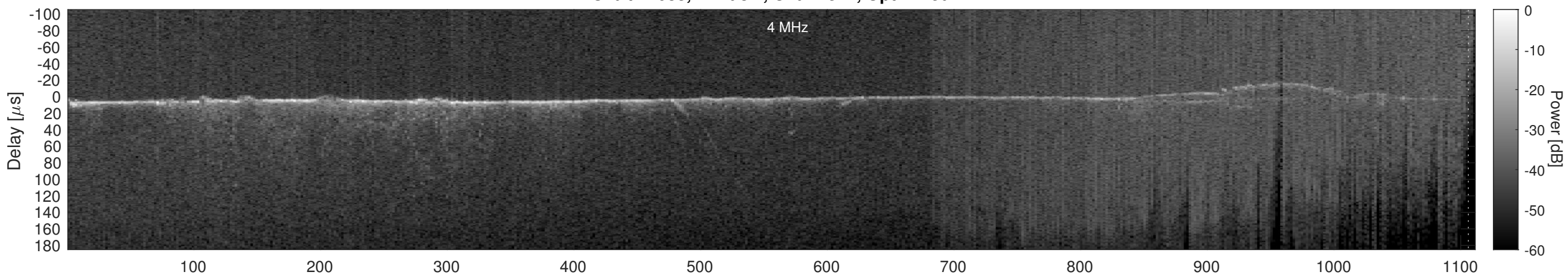
Orbit 12083, Cluttergram
