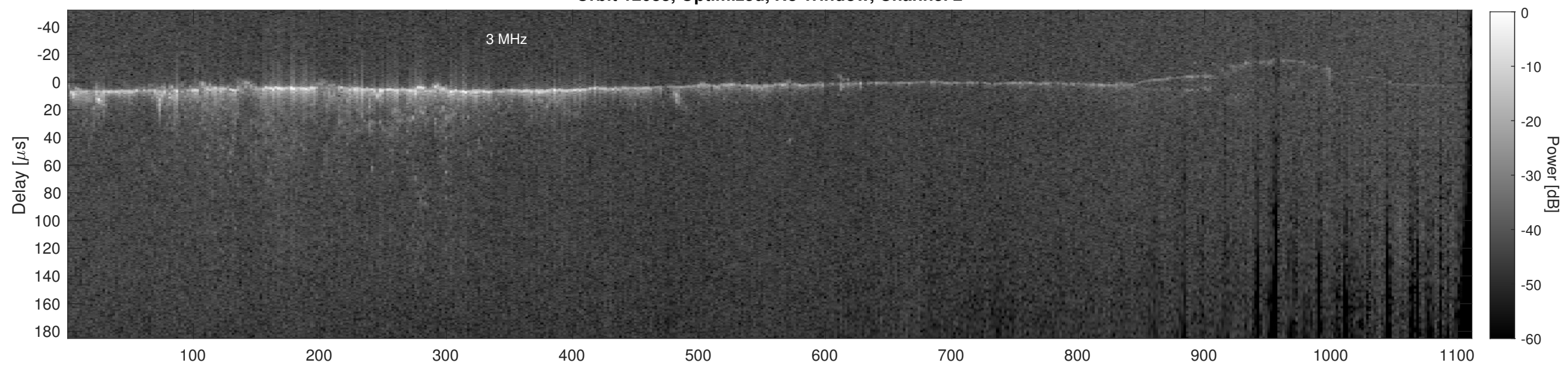
Orbit 12083, Cluttergram
