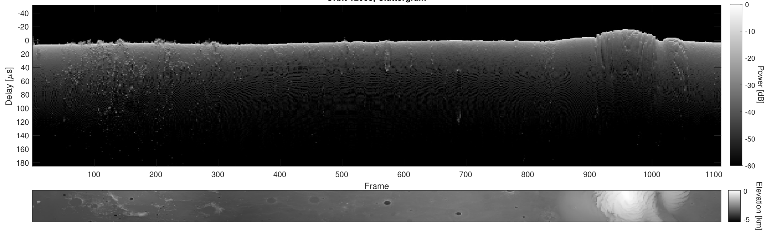
Orbit 12083, Cluttergram
