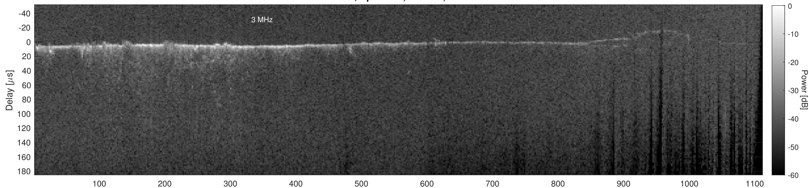
Orbit 12083, Cluttergram
