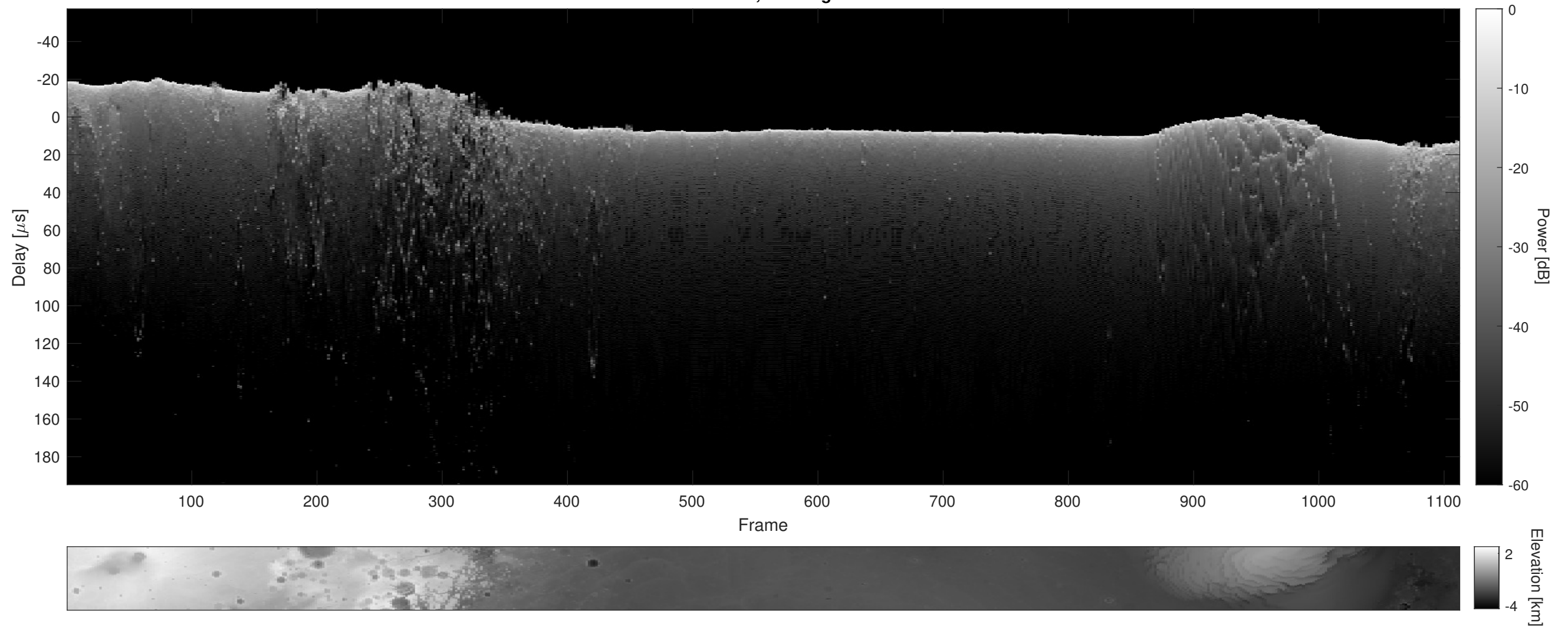
Orbit 12084, Cluttergram
