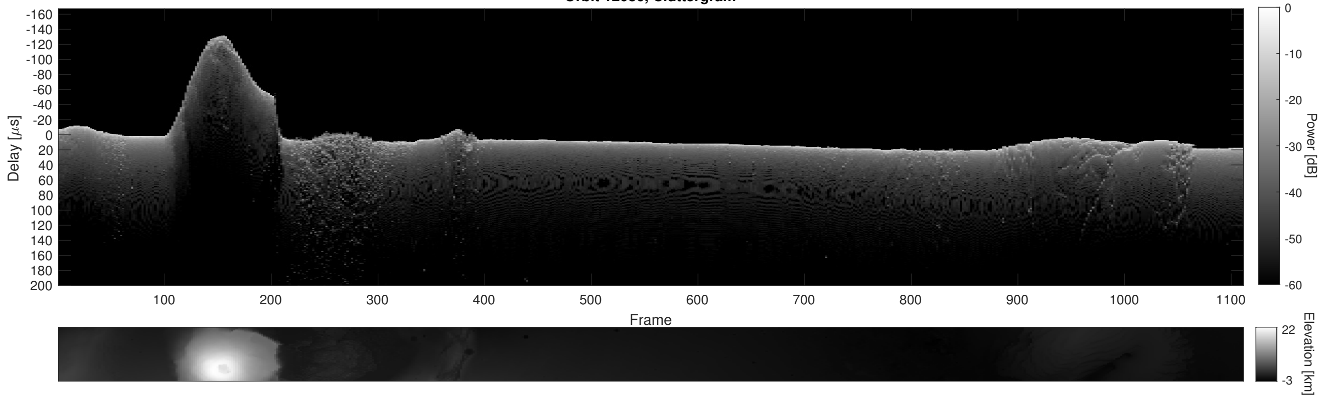
Orbit 12086, Cluttergram
