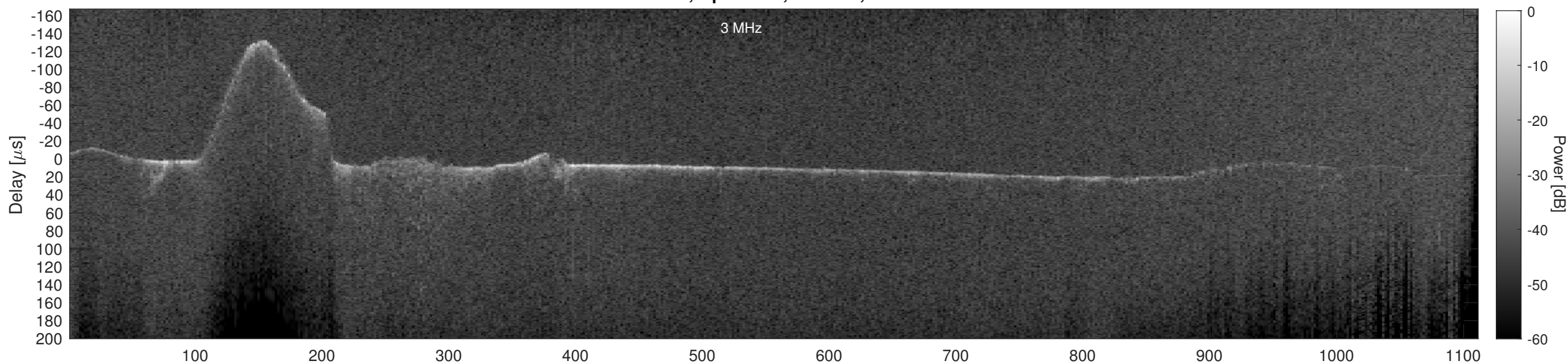
Orbit 12086, Cluttergram
