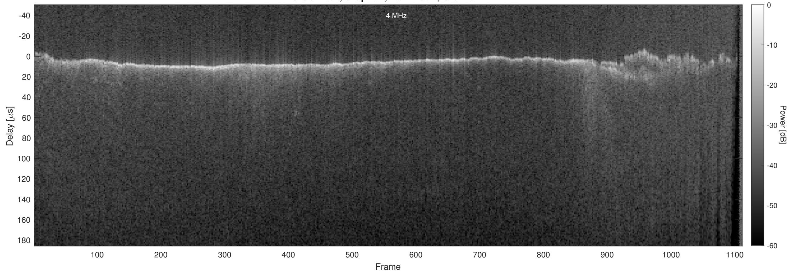
Orbit 12087, Chapman, No Window, Channel 2
