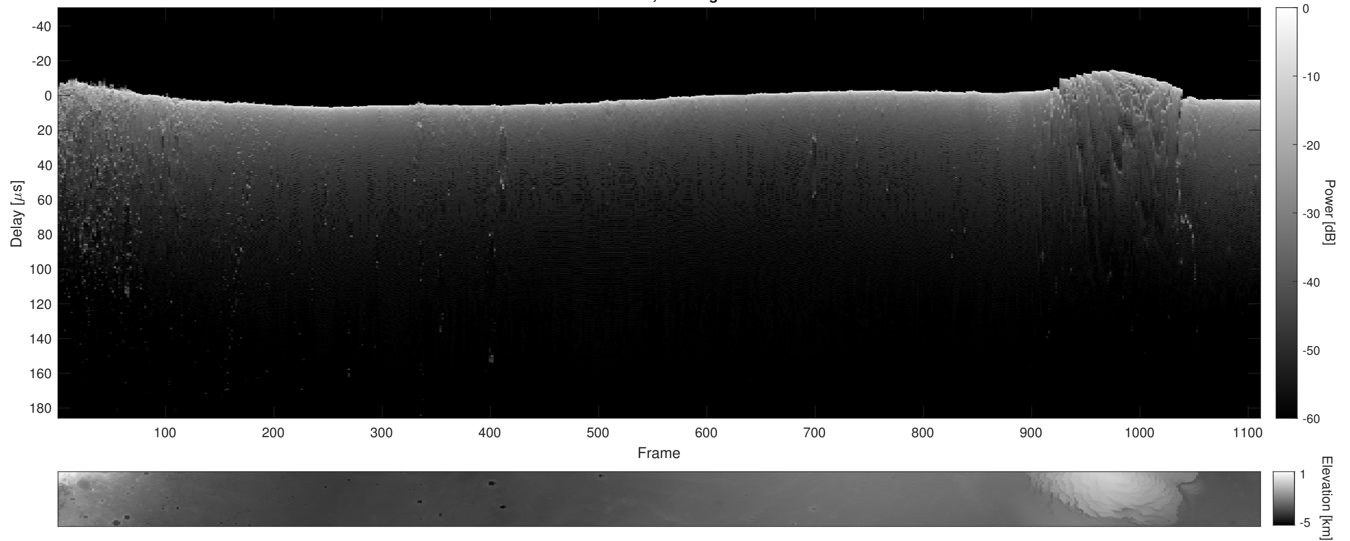
Orbit 12087, Cluttergram
