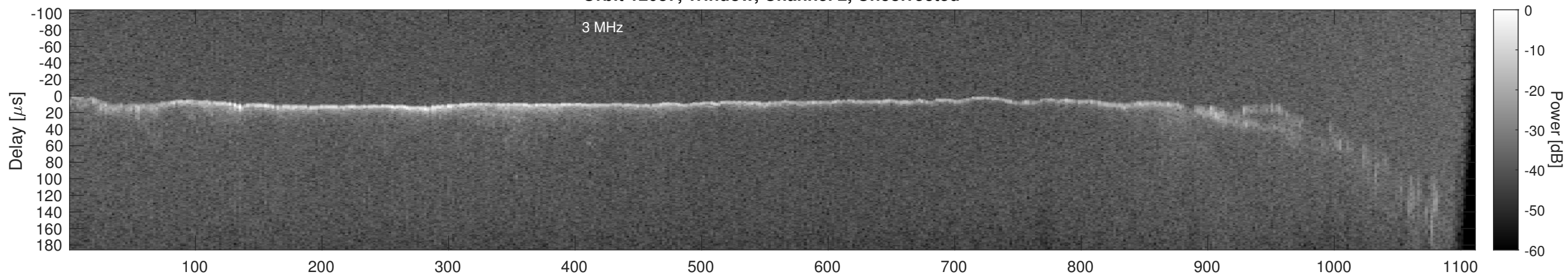
Orbit 12087, Window, Channel 2, Chapman
