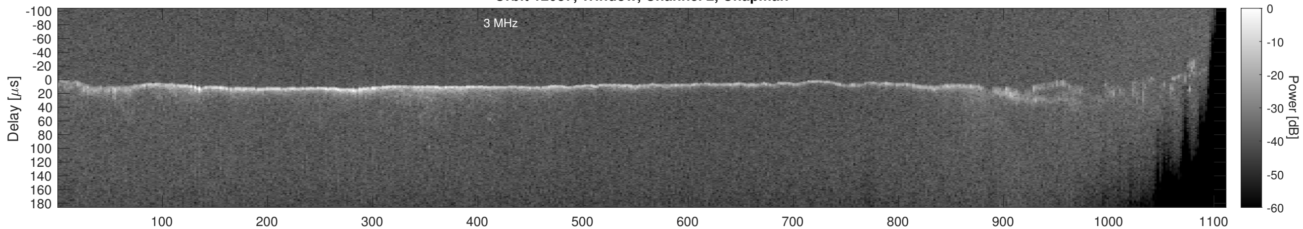
Orbit 12087, Window, Channel 2, Optimized
