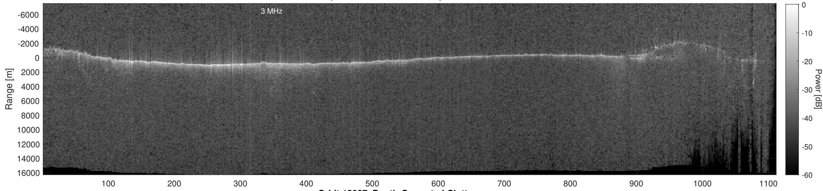
Orbit 12087, Depth-Corrected Cluttergram
