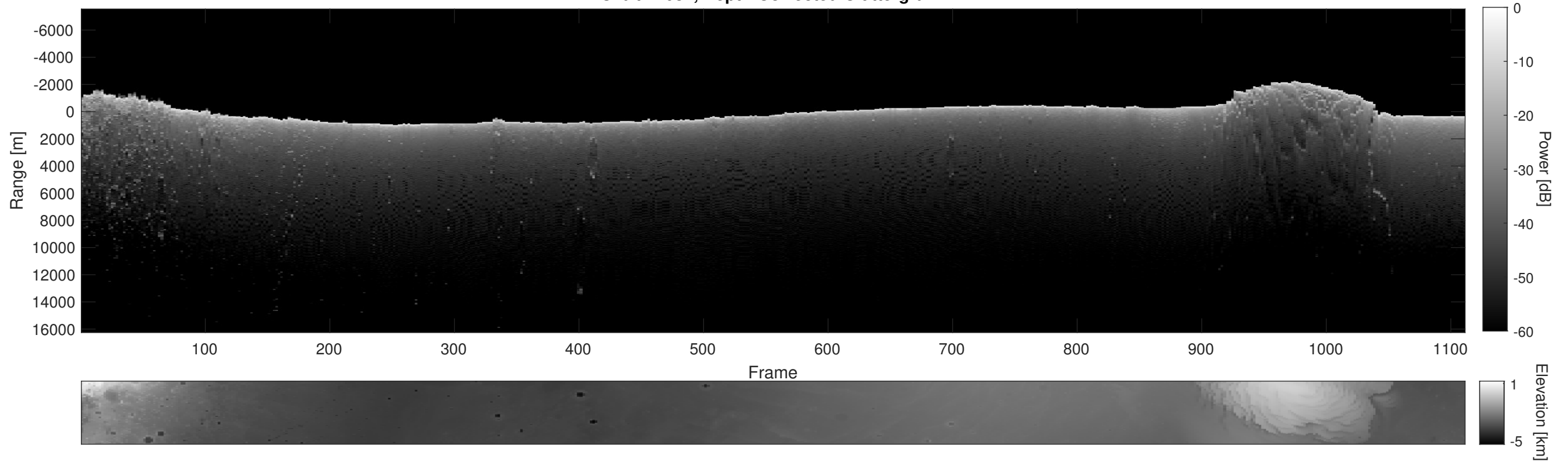
Orbit 12087, Depth-Corrected Cluttergram
