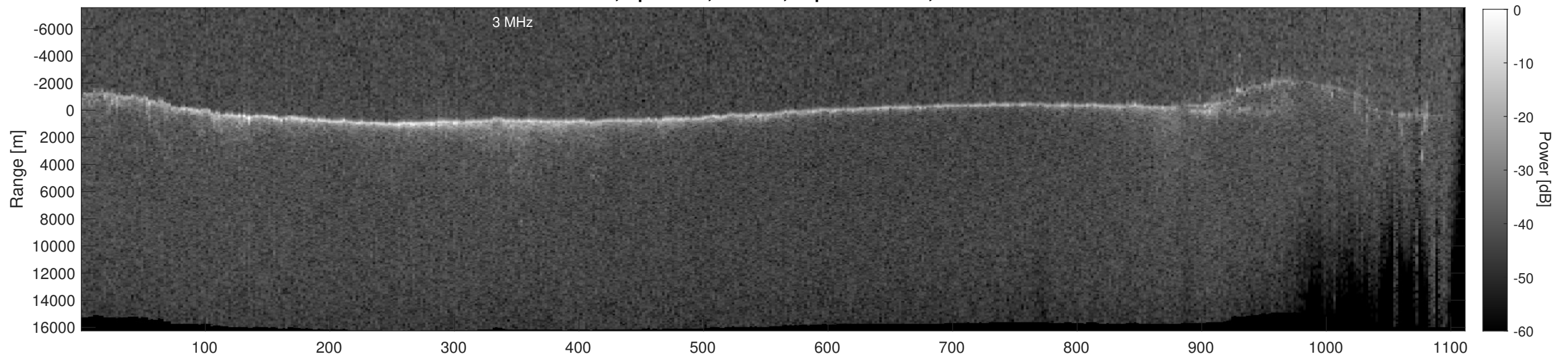
Orbit 12087, Depth-Corrected Cluttergram
