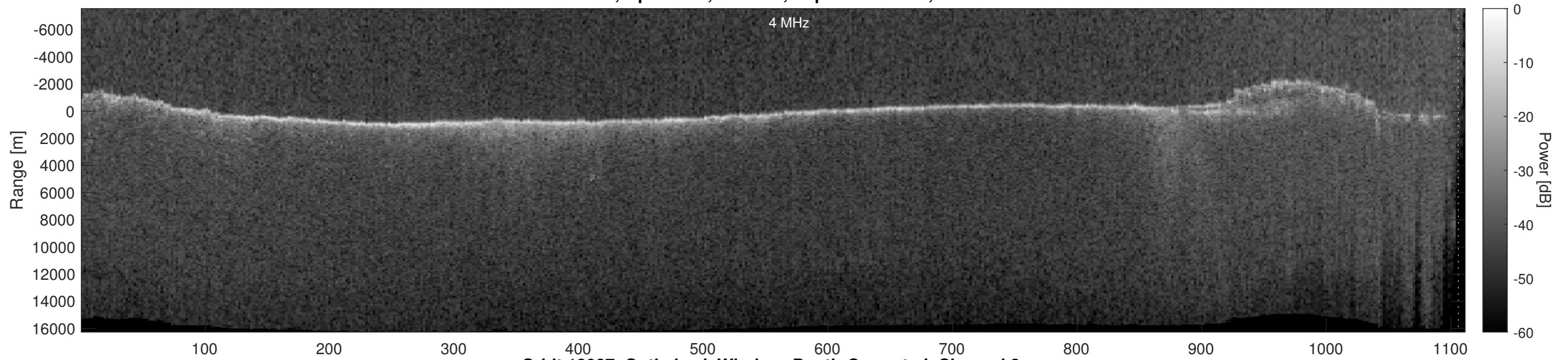
Orbit 12087, Optimized, Window, Depth-Corrected, Channel 2
