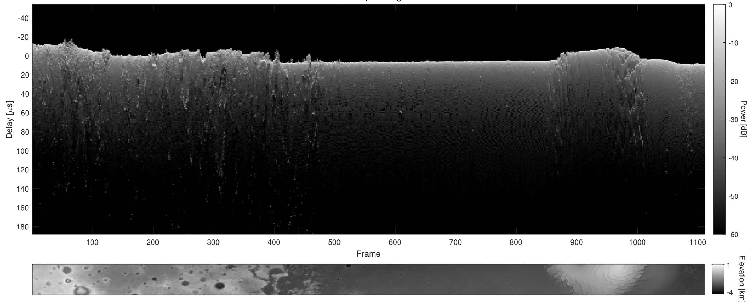
Orbit 12088, Cluttergram
