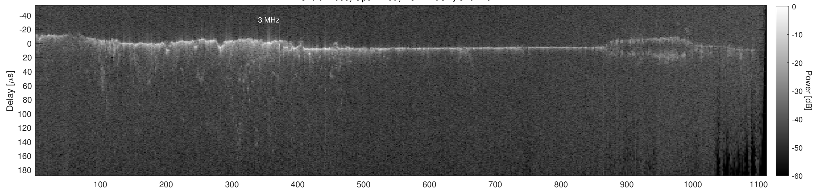
Orbit 12088, Cluttergram
