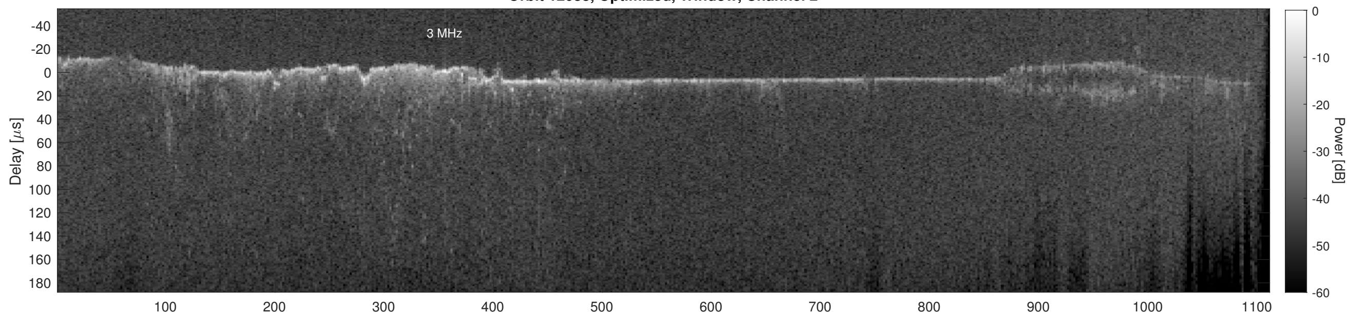
Orbit 12088, Cluttergram
