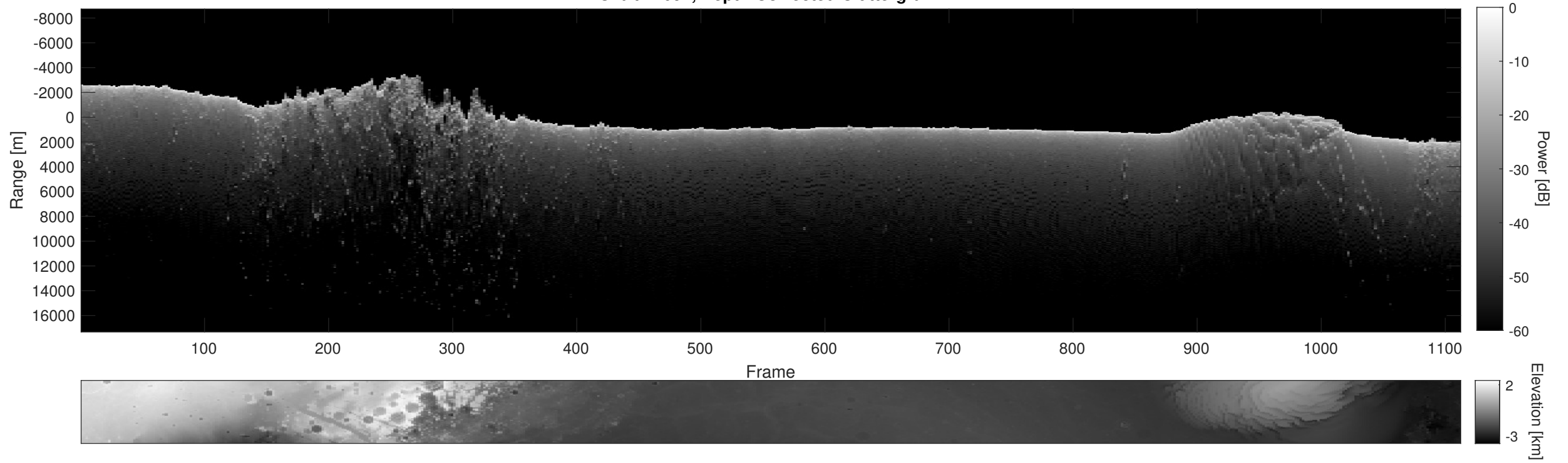
Orbit 12091, Depth-Corrected Cluttergram
