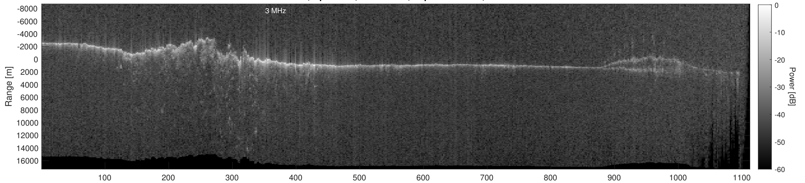
Orbit 12091, Depth-Corrected Cluttergram
