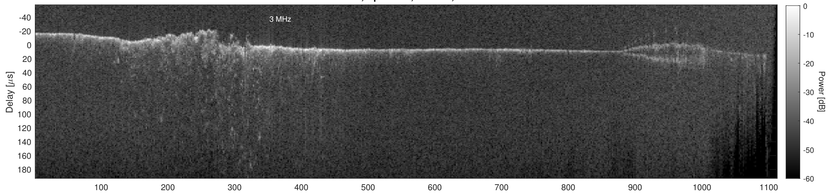
Orbit 12091, Cluttergram
