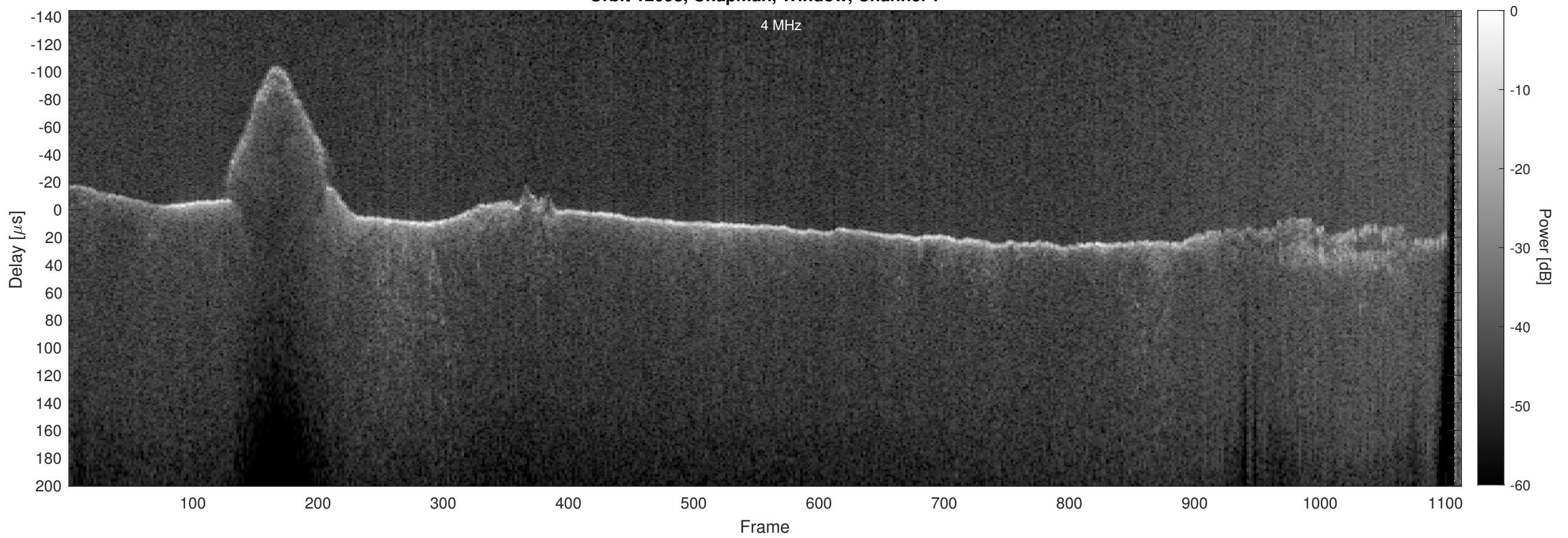
Orbit 12093, Chapman, Window, Channel 2
