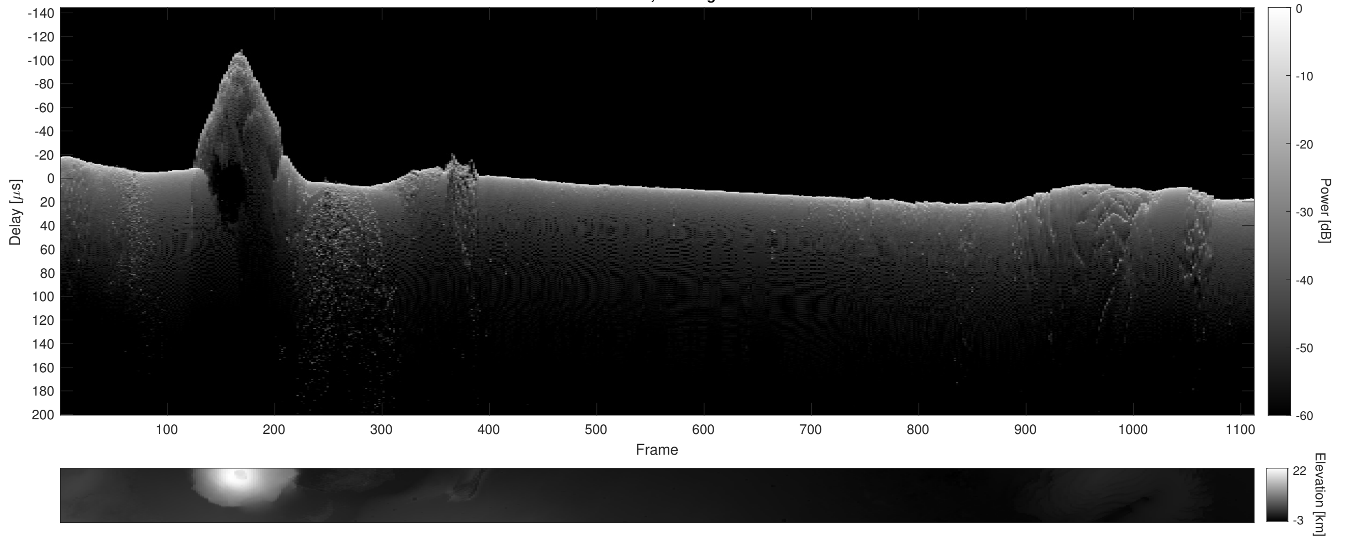
Orbit 12093, Cluttergram
