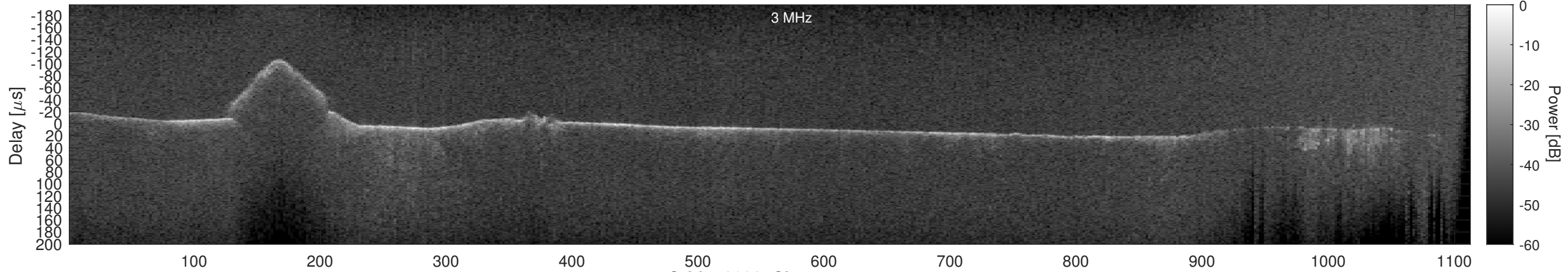
Orbit 12093, Cluttergram
