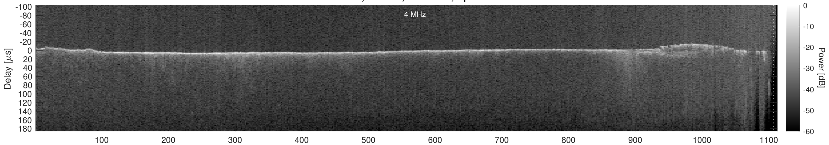
Orbit 12094, Cluttergram
