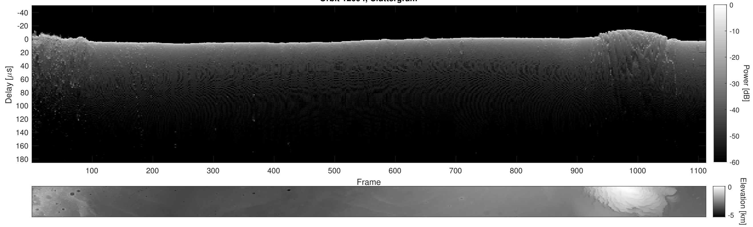
Orbit 12094, Cluttergram
