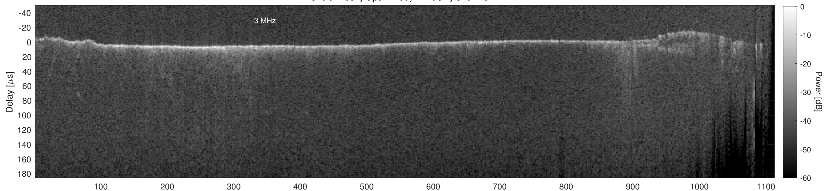
Orbit 12094, Cluttergram
