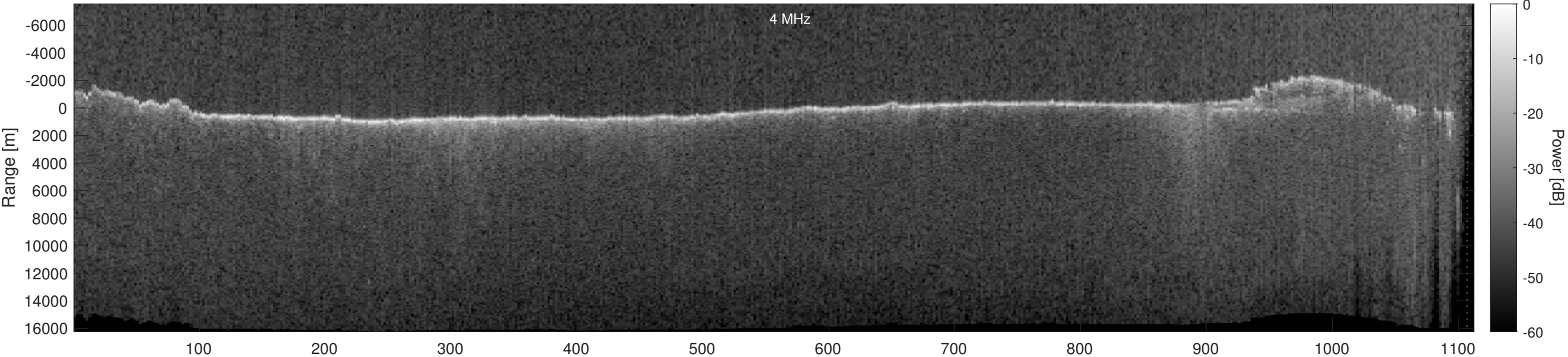
Orbit 12094, Optimized, Window, Depth-Corrected, Channel 2
