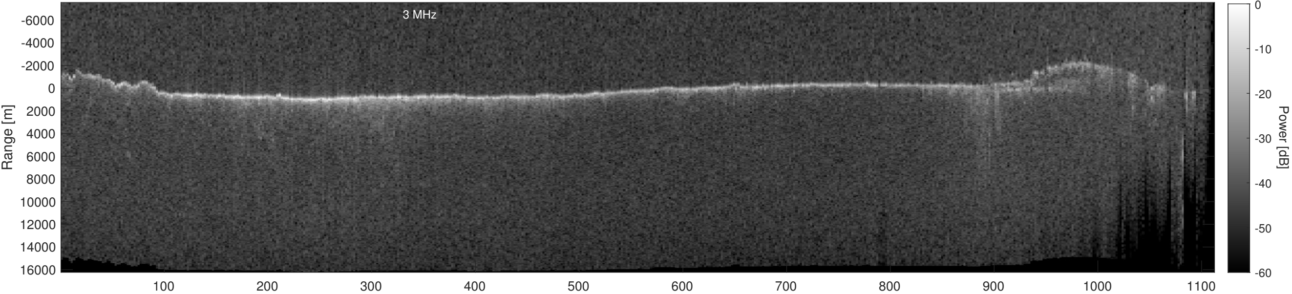
Orbit 12094, Depth-Corrected Cluttergram
