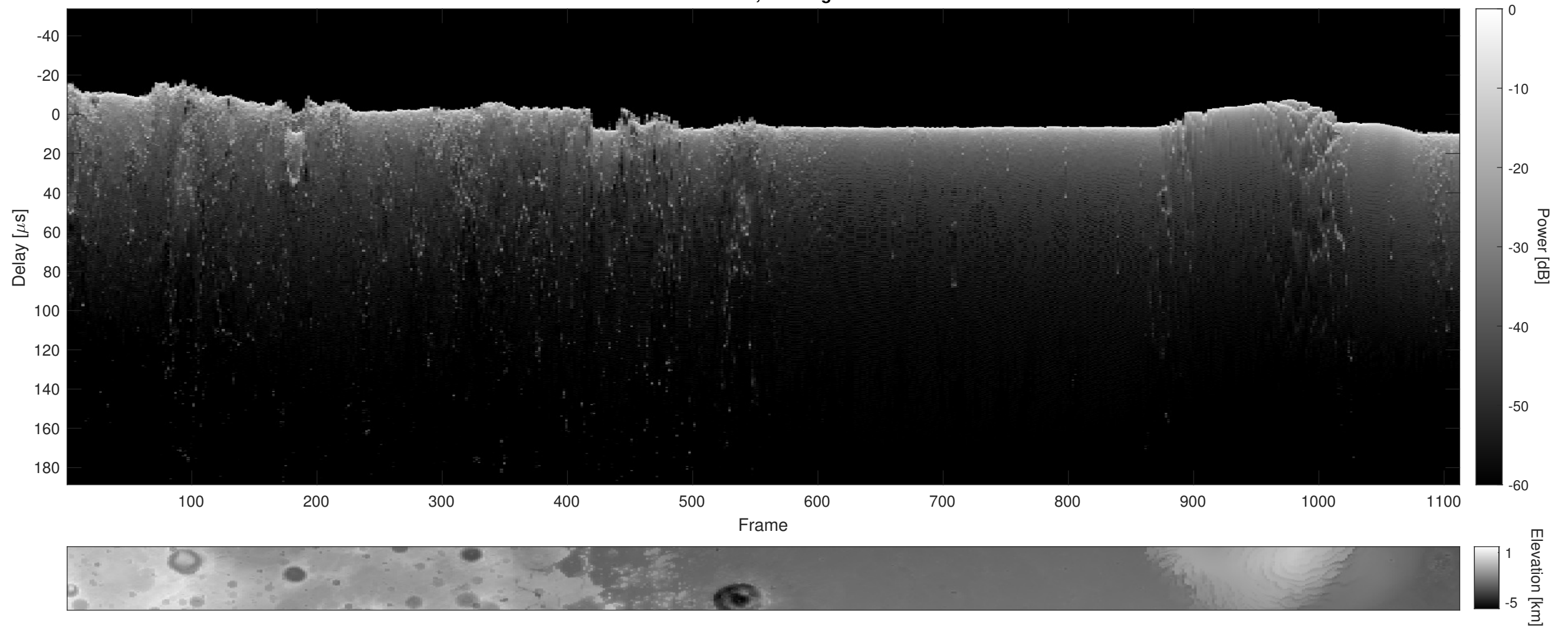
Orbit 12095, Cluttergram
