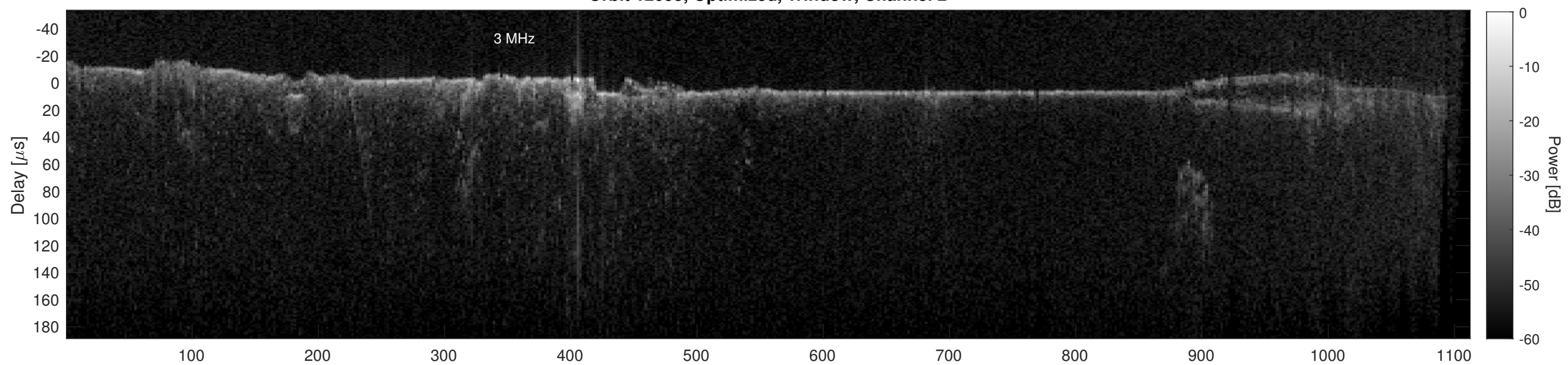
Orbit 12095, Cluttergram
