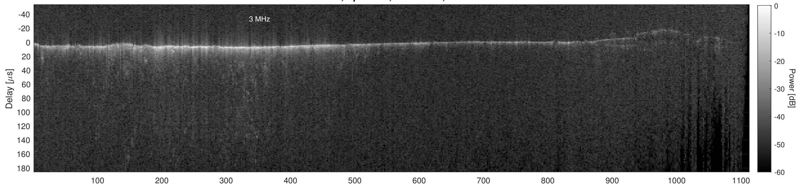
Orbit 12097, Cluttergram
