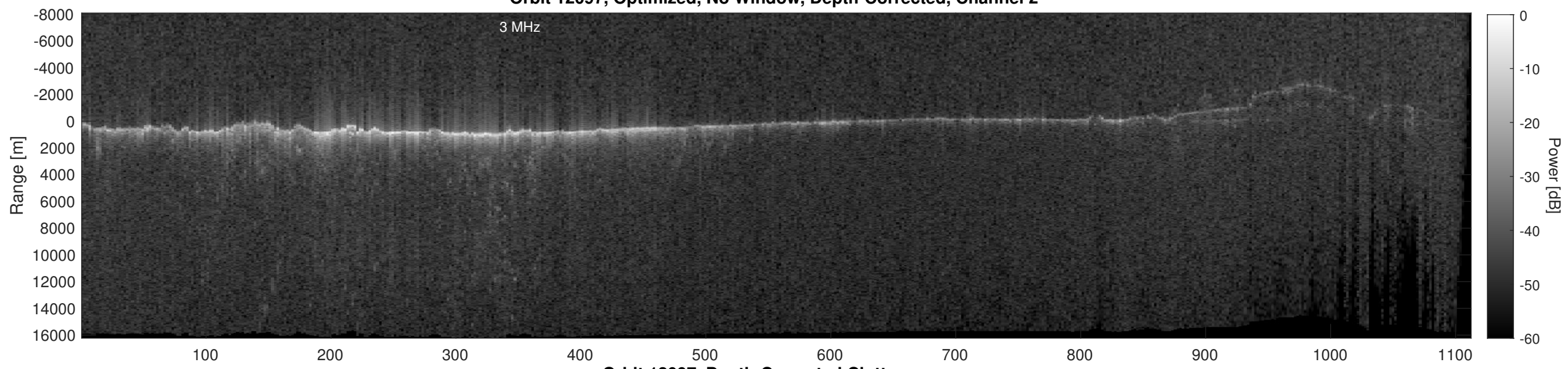
Orbit 12097, Depth-Corrected Cluttergram
