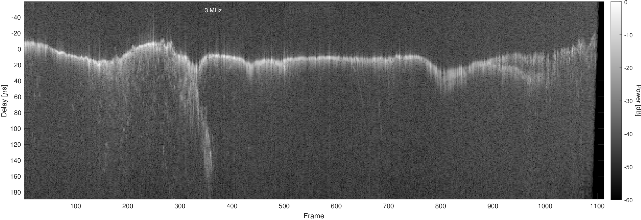
Orbit 12098, Chapman, No Window, Channel 2
