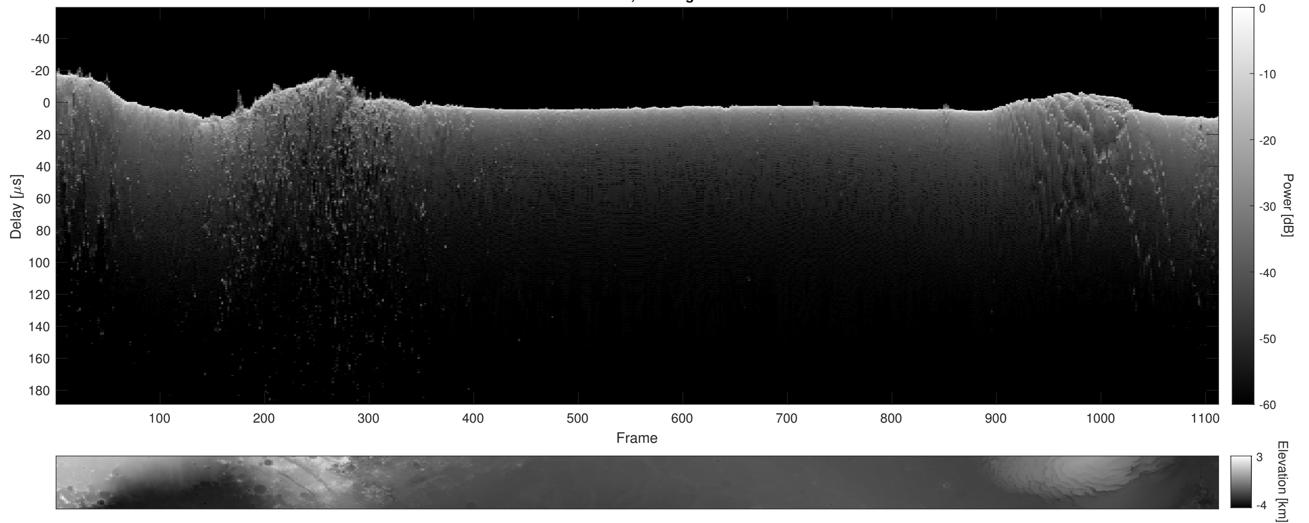
Orbit 12098, Cluttergram
