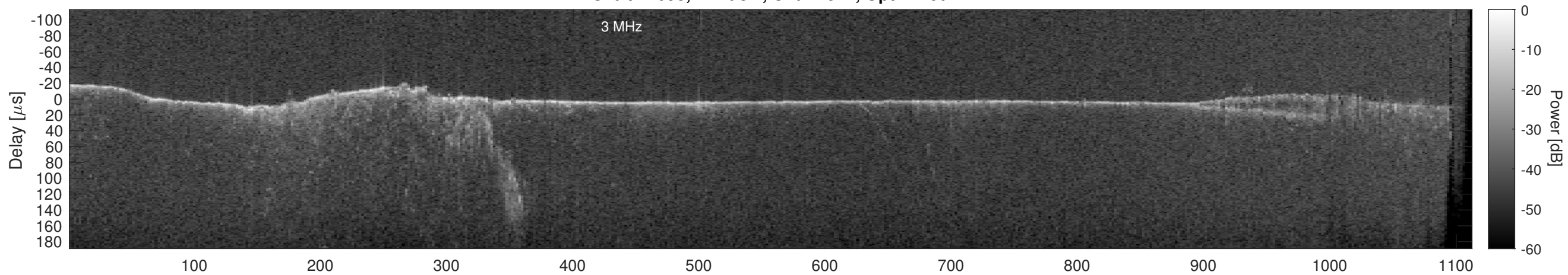
Orbit 12098, Cluttergram
