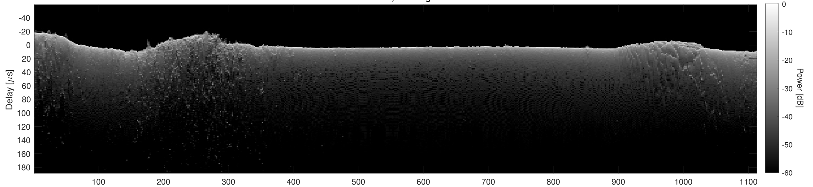
Orbit 12098, Cluttergram
