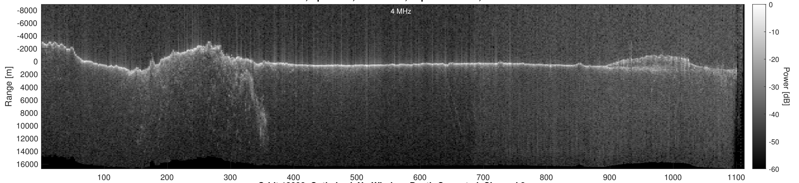
Orbit 12098, Optimized, No Window, Depth-Corrected, Channel 2
