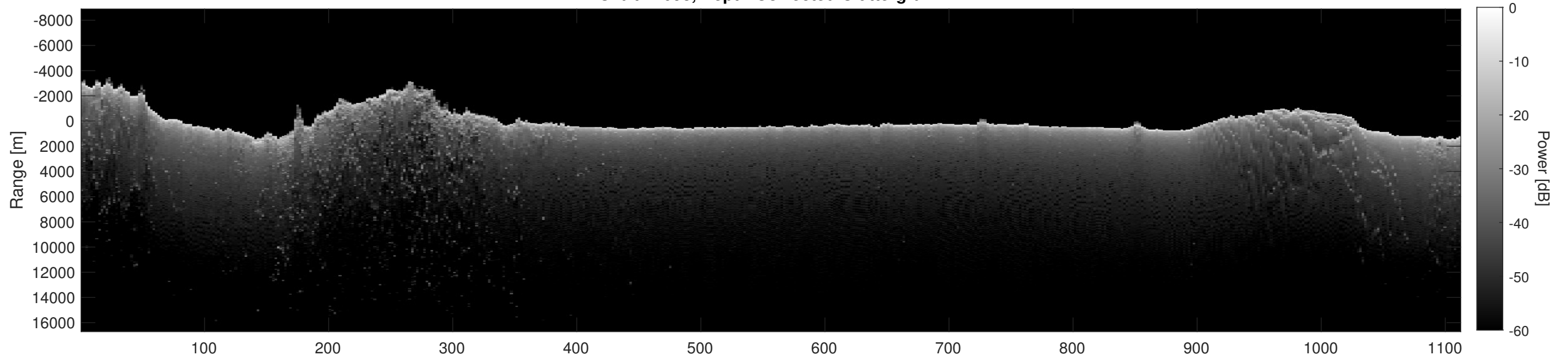
Orbit 12098, Depth-Corrected Cluttergram
