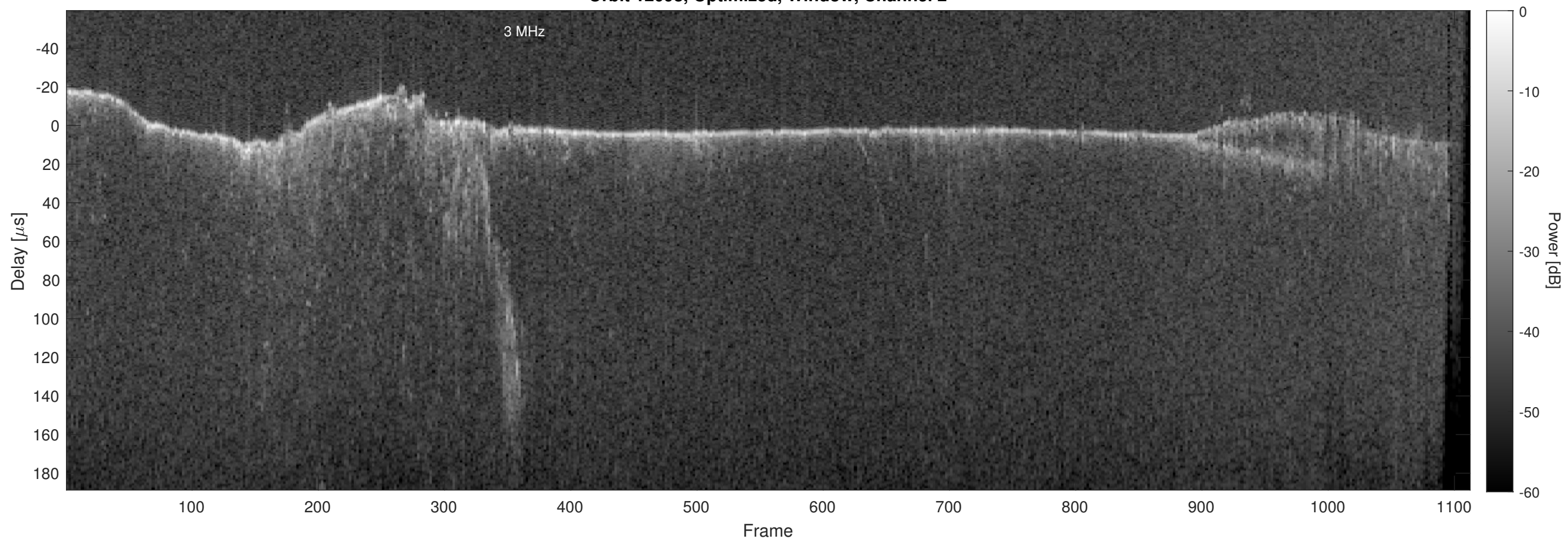
Orbit 12098, Optimized, Window, Channel 2
