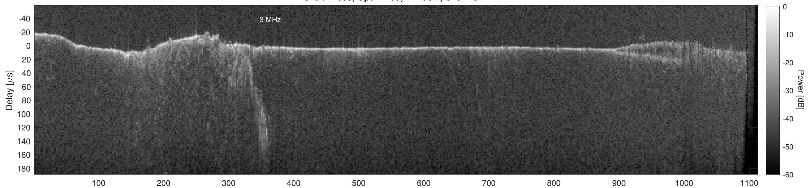
Orbit 12098, Cluttergram
