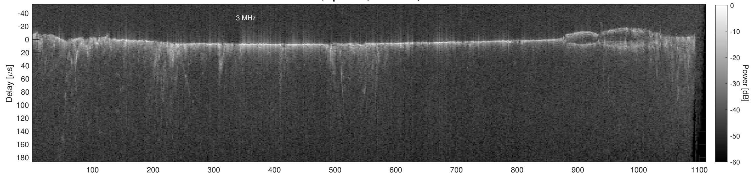
Orbit 12099, Cluttergram
