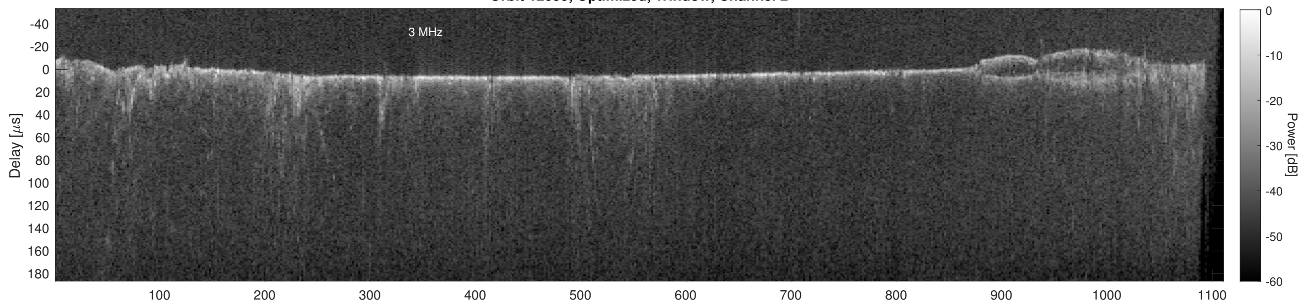
Orbit 12099, Cluttergram
