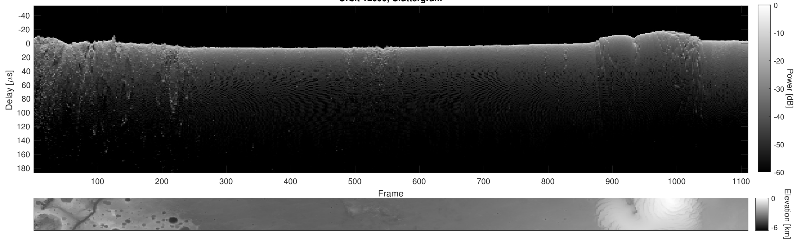
Orbit 12099, Cluttergram
