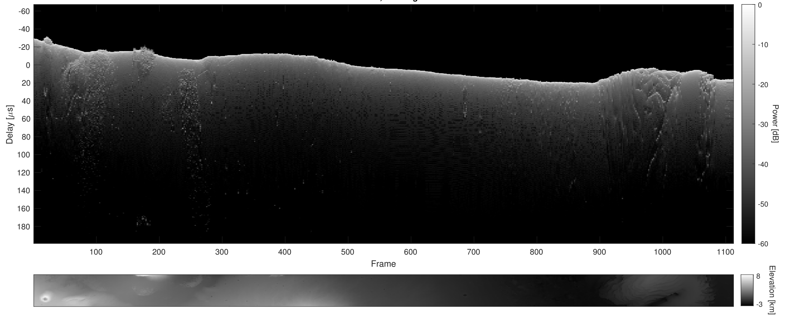
Orbit 12100, Cluttergram
