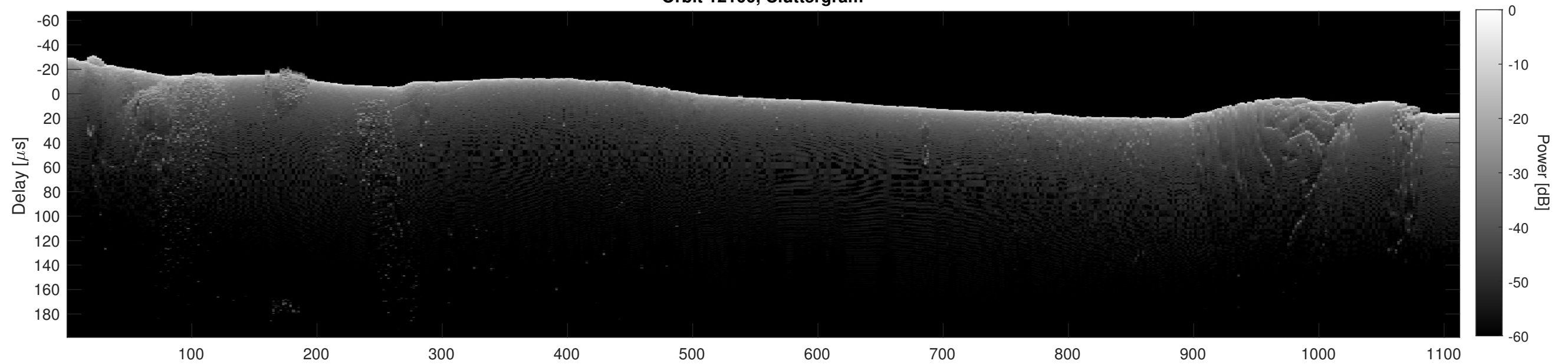
Orbit 12100, Cluttergram
