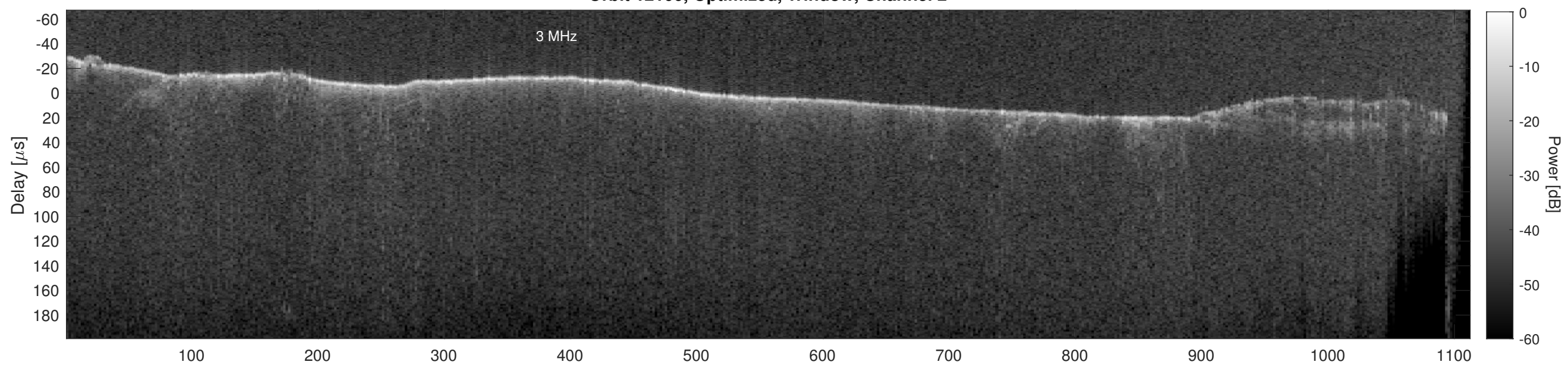
Orbit 12100, Cluttergram
