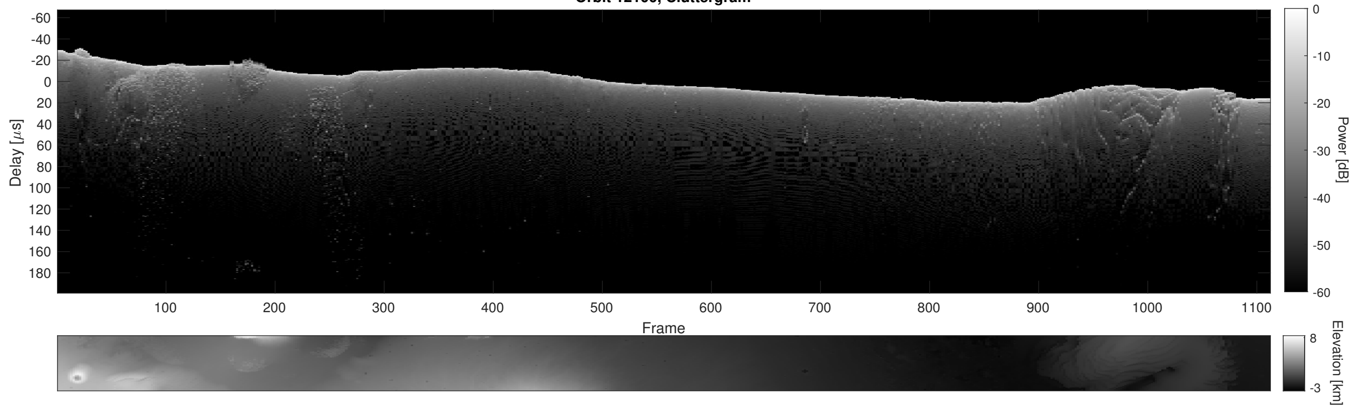
Orbit 12100, Cluttergram
