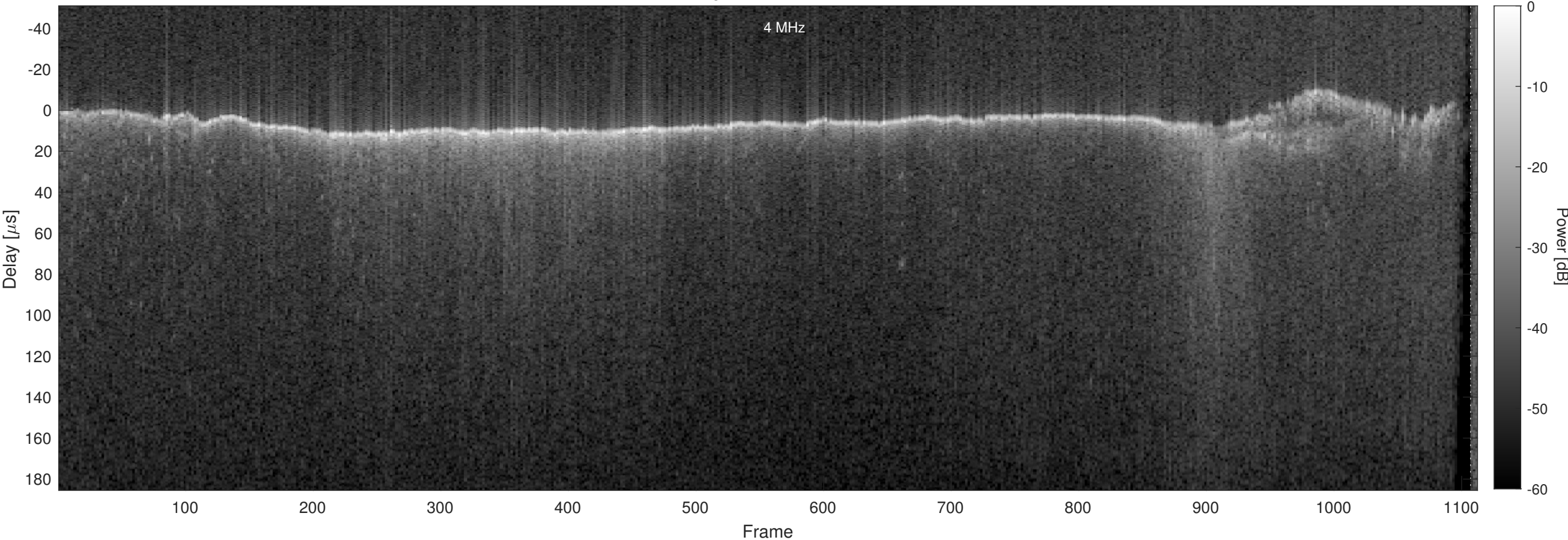
Orbit 12101, Chapman, No Window, Channel 2
