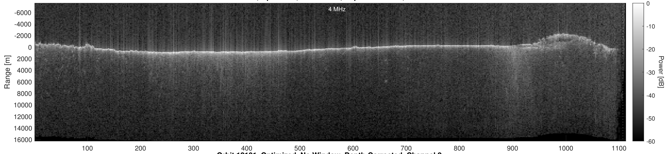
Orbit 12101, Optimized, No Window, Depth-Corrected, Channel 2
