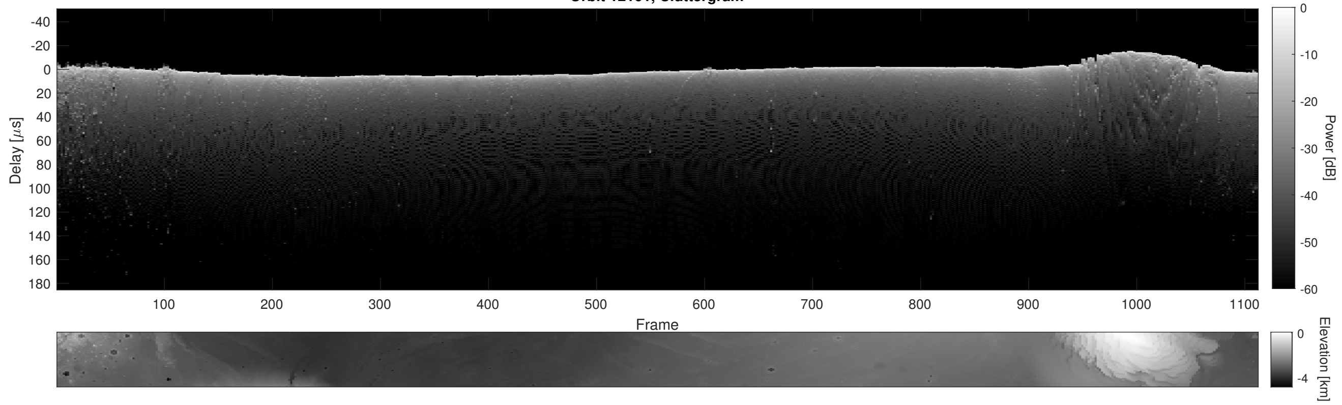
Orbit 12101, Cluttergram
