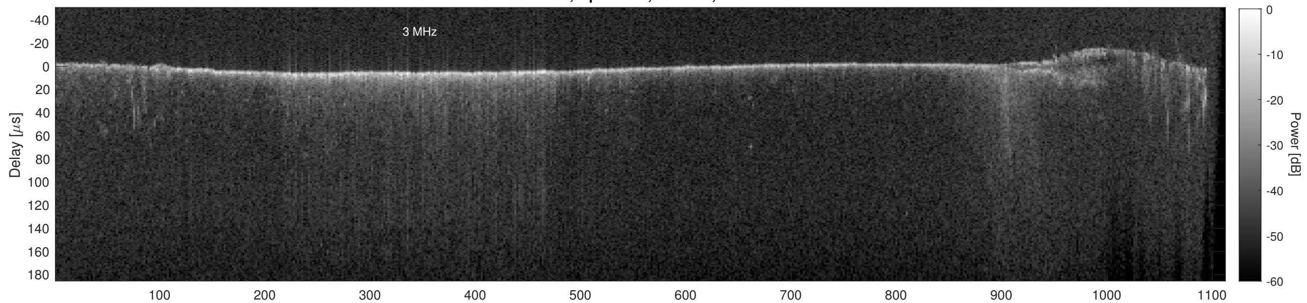
Orbit 12101, Cluttergram
